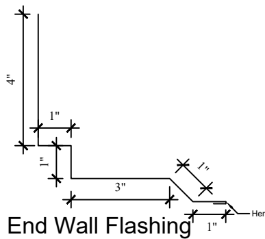
4600 Universal End Wall
