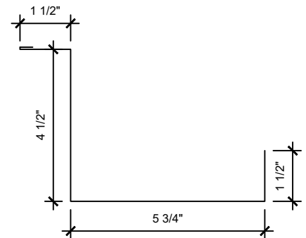
Porch Beam Trim
