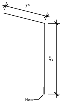
#31 Eave Trim
