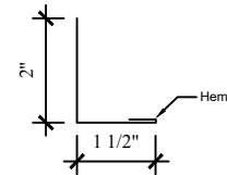
6C 1 1/2 X 2 Side Overhang
