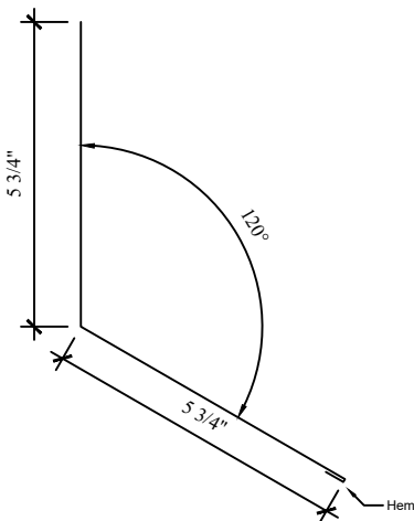
Universal End Wall Flashing
