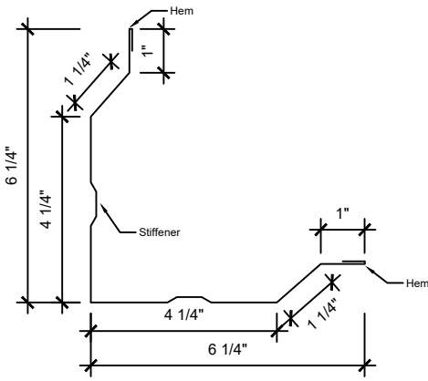
22 Corner Trim
