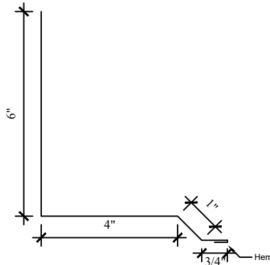
Side Wall Flashing
