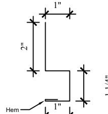
33 Base Trim
