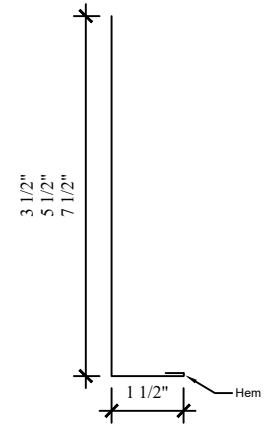
Door Post Trim
