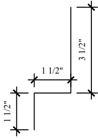
RC5 Track Filler
